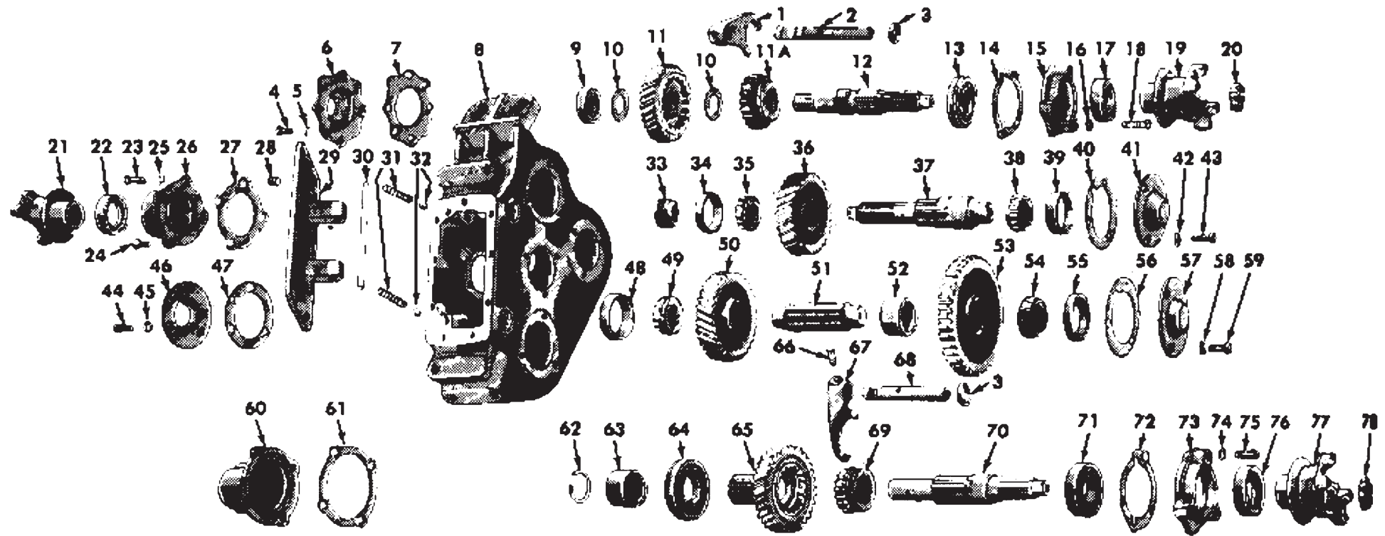
Timken model 221 transfer case (© G.M.C.)
